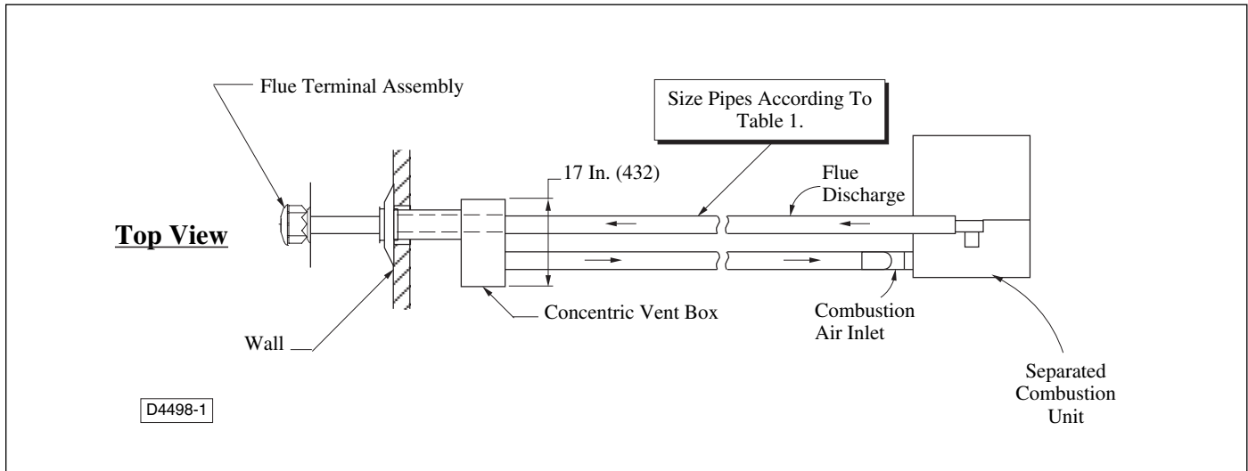
Figure 3– Typical Horizontal Vent Kit Installation Requirements
